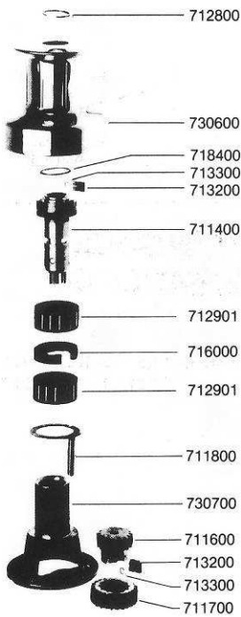
No. 28 Two Speed Winch
