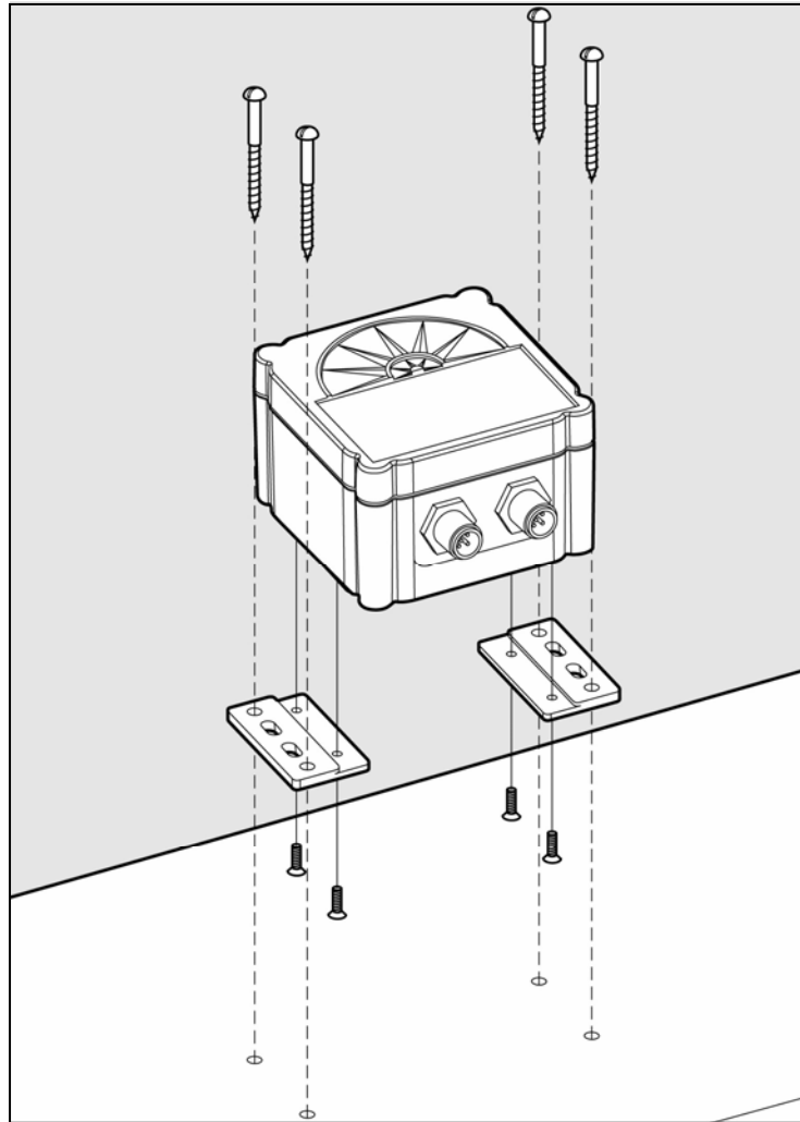
Figure 1 – Mounting the SSC200 to a Horizontal Surface
