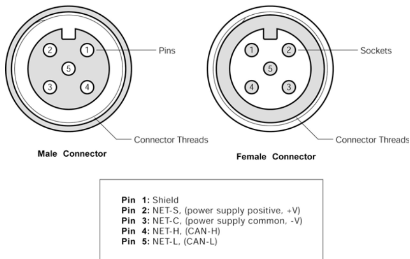
Figure 6 – NMEA 2000® Connector Face Views
