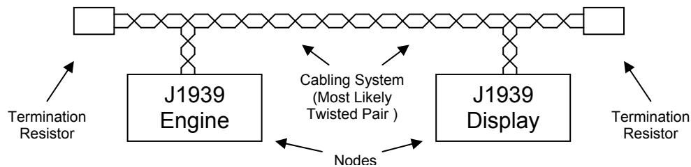
Figure 2 - Typical Single Engine J1939 Network
