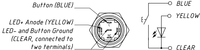
Figure 2. Button terminals and electrical scheme
