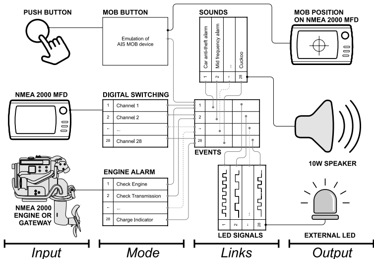
Figure 1. Functional scheme
