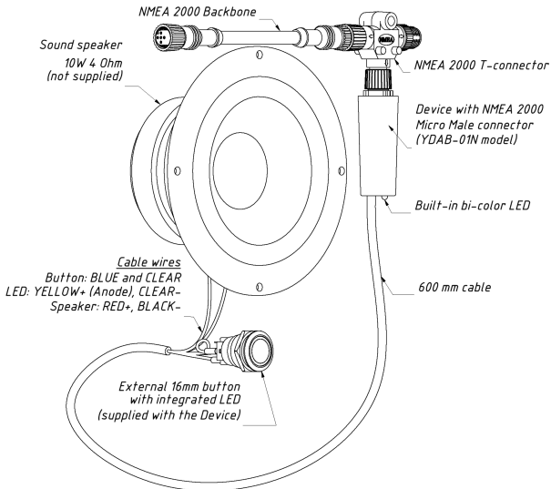
Figure 1. Device connection
